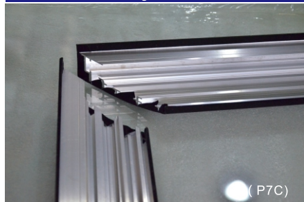
Connector connecting method of 100B (Picture 4C, 5C, 6C)
